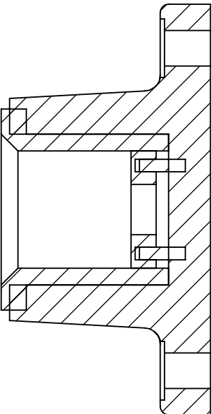
SECTION C-C SCALE 1 : 2
